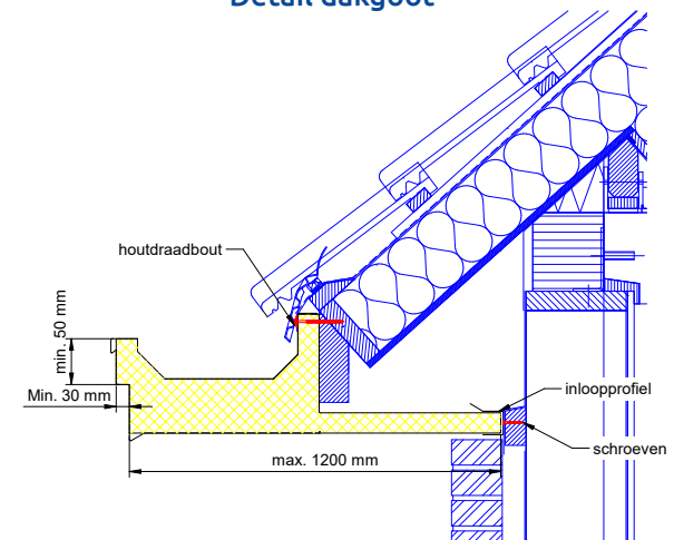
Detail dakgoot
