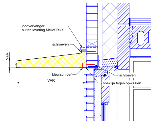
Detail luifel
