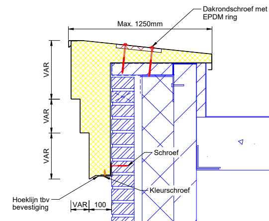
Detail dakrand
